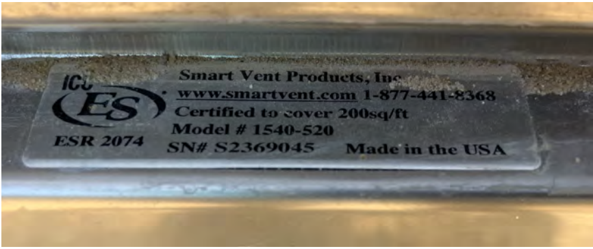
ENGINEERED FLOOD VENT MODEL NUMBER
